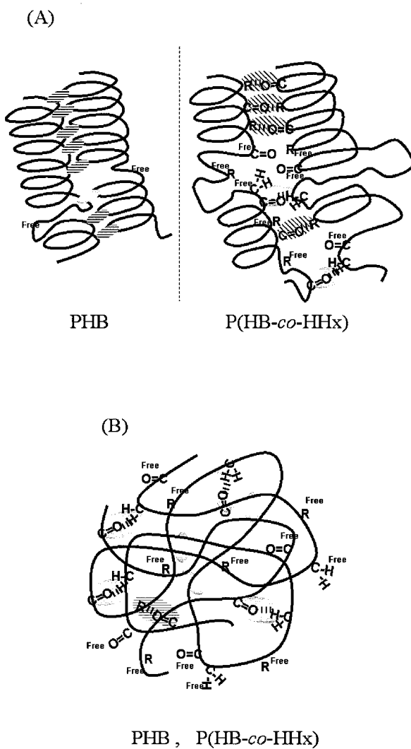
Figure 11. (A) Proposed helical structure models for PHB and P(HB-co-HHx). (B) Proposed amorphous structure model for PHB and P(HB-co-HHx).
